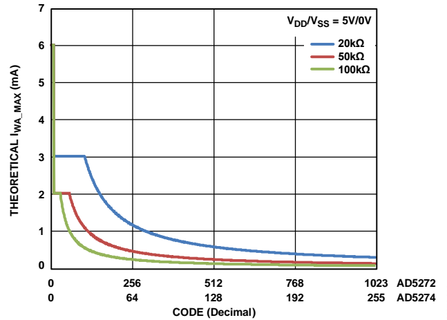
Figure 27. Theoretical Maximum Current vs. Code
