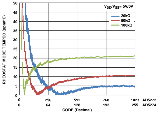
Figure 24. Tempco \Delta R_{WA}/\Delta T vs. Code
