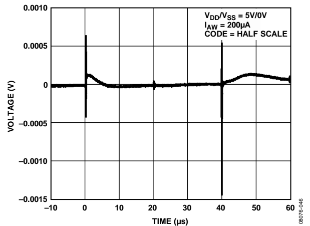
Figure 34. Digital Feedthrough
