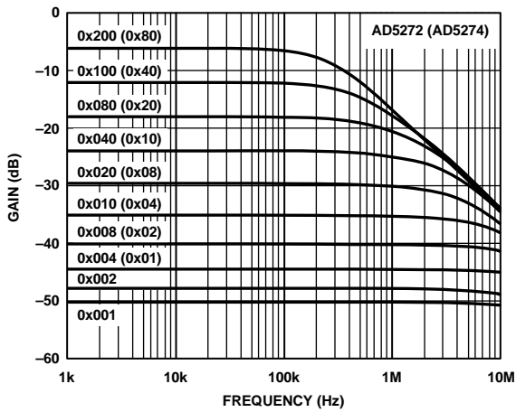
Figure 25. 20 kΩ Gain vs. Code vs. Frequency
