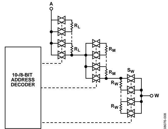
Figure 46. Simplified RDAC Circuit
