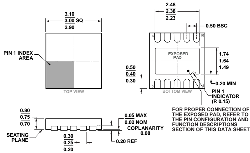
Figure 50. 10-Lead Frame Chip Scale Package [LFCSP_WD] 3 mm x 3 mm Body, Very Thin, Dual Lead (CP-10-9) Dimensions shown in millimeters
