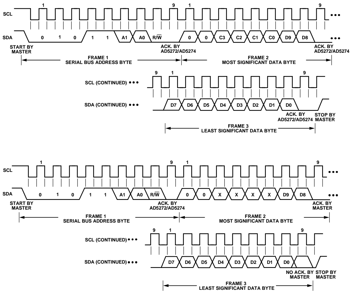
Figure 45. Read Command
