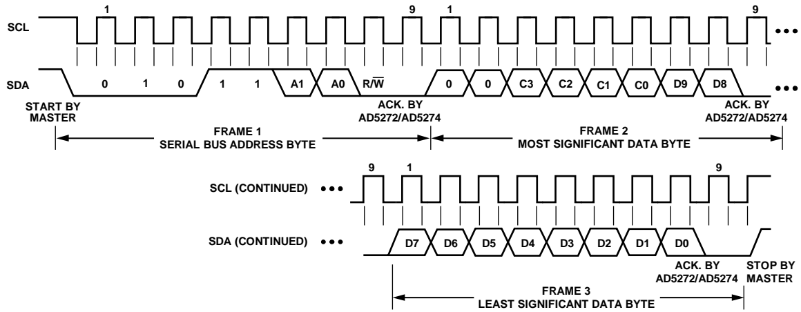
Figure 43. Write Command
