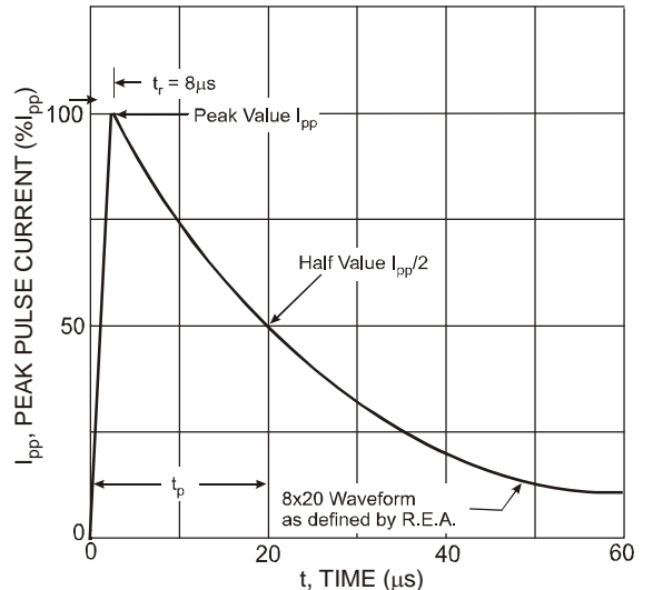
Fig. 2 Pulse Waveform
