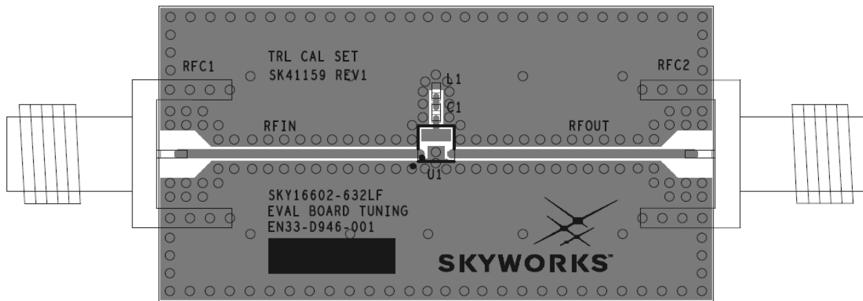
Figure 11. SKY16602-632LF Evaluation Board Assembly Diagram (Tuned Circuit)
