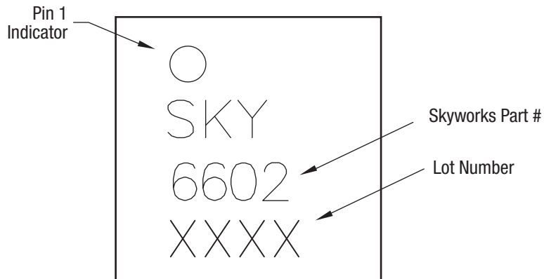
Figure 14. SKY16602-632LF Typical Case Markings
