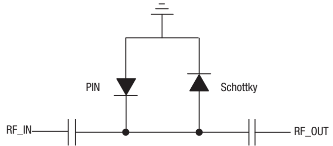
Figure 1. SKY16602-632LF Block Diagram
