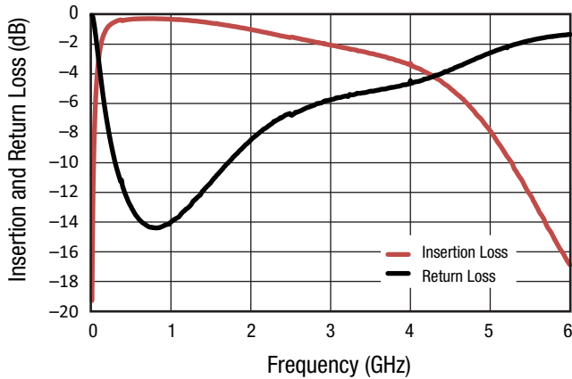
Figure 4. Small Signal Performance without External Tuning
