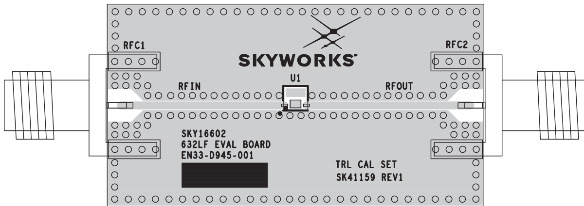
Figure 10. SKY16602-632LF Evaluation Board Assembly Diagram
