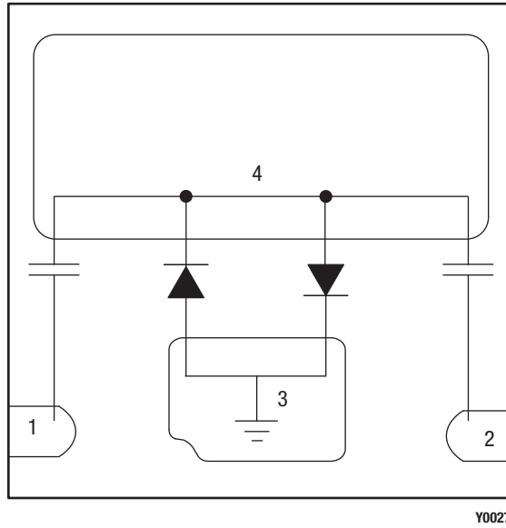
Figure 2. SKY16602-632LF Pinout, 2-Pin MLP (Top View)
