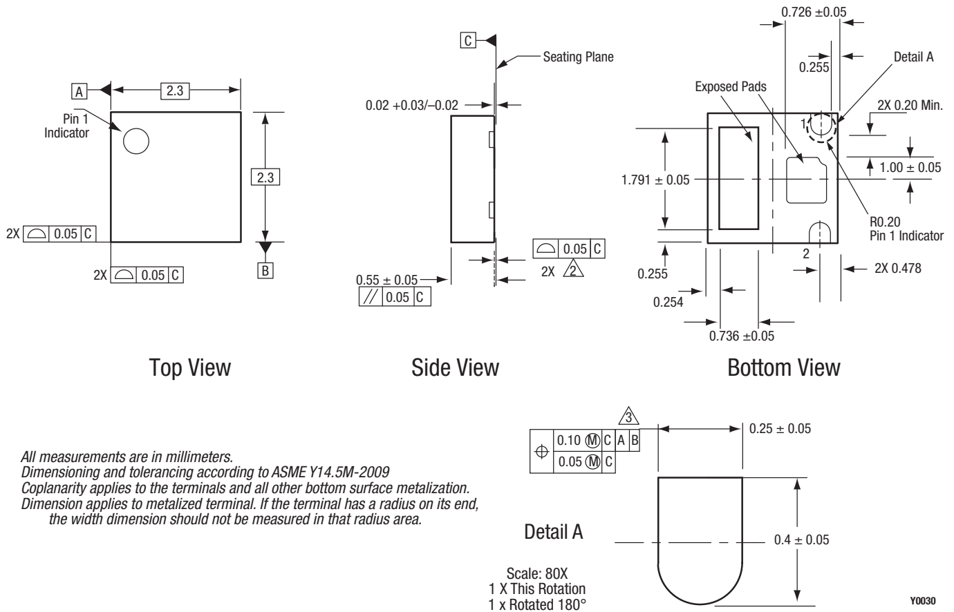
Figure 15. SKY16602-632LF 2-PIN MLP Package Dimensions
