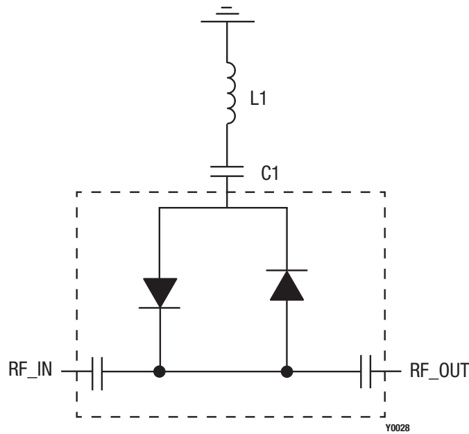
Figure 3. SKY16602-632LF Schematic with External Tuning Networks Optimized for 2.45 GHz
