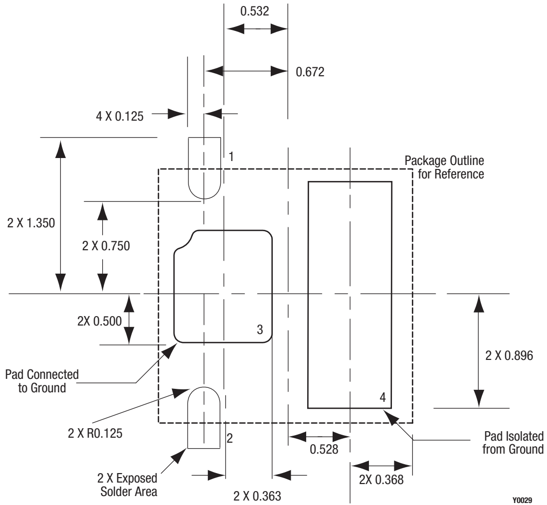
Figure 13. SKY16602-632LF PCB Layout Footprint
