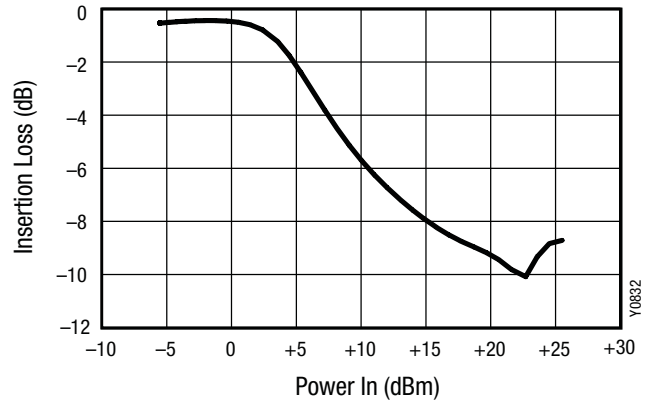
Figure 7. Insertion Loss vs CW Input Power at 2.45 GHz (Tuned Circuit)
