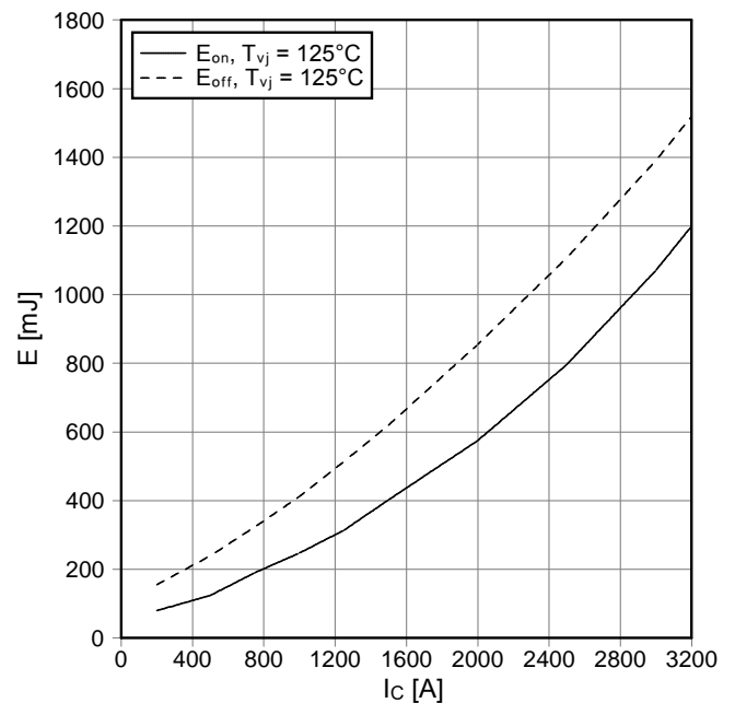
Schaltverluste IGBT-Wechselr. (typisch) switching losses IGBT-inverter (typical) E_{on} = f(I_C) , E_{off} = f(I_C) V_{GE} = \pm 15\text{ V} , R_{Gon} = 0.9\ \Omega , R_{Goff} = 0.9\ \Omega , V_{CE} = 900\text{ V}
