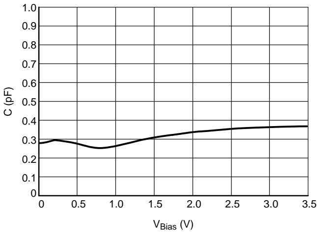
Figure 1. CV Characteristics
