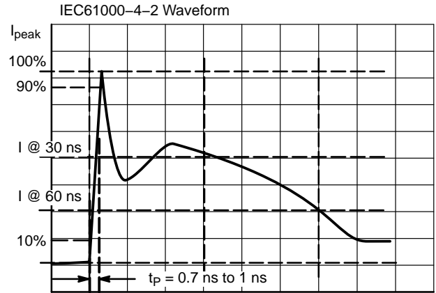
Figure 8. IEC61000-4-2 Spec
